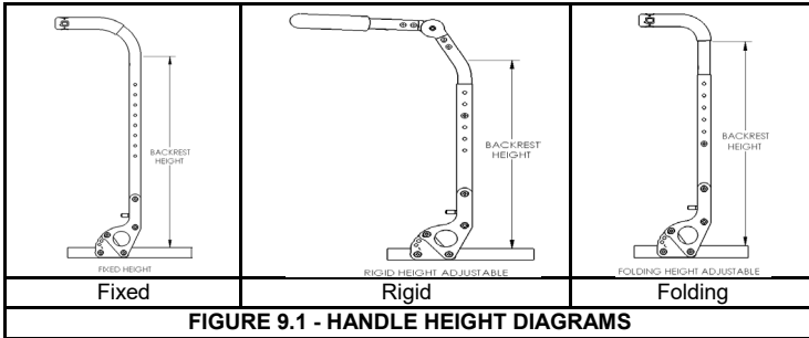
FIGURE 9.1 - HANDLE HEIGHT DIAGRAMS
